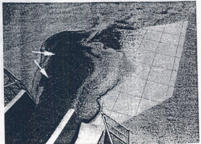
Figure 2. Deposit from unsaturated flow. Note arcuate ridges on surface.
