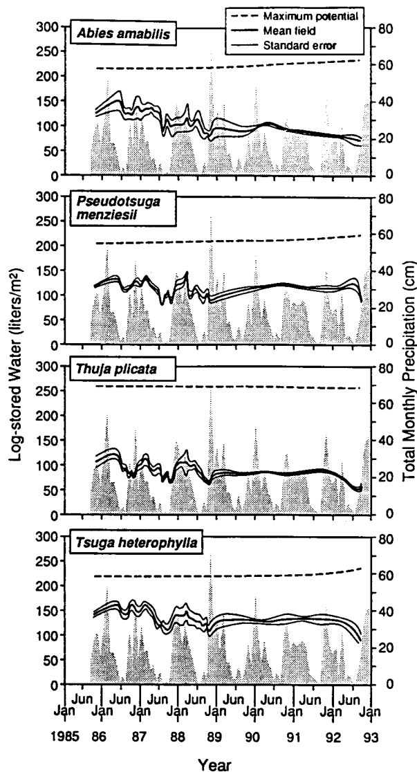
Fig. 4. Mean waterstores in four species of conifer logs during the first 8 years of decomposition. Precipitation data, shown as a gray histogram, is from the Primary Meteorological Station, H J Andrews Experimental Forest (Bierlmaier and McKee, 1989). (Original data is available from the senior author).
