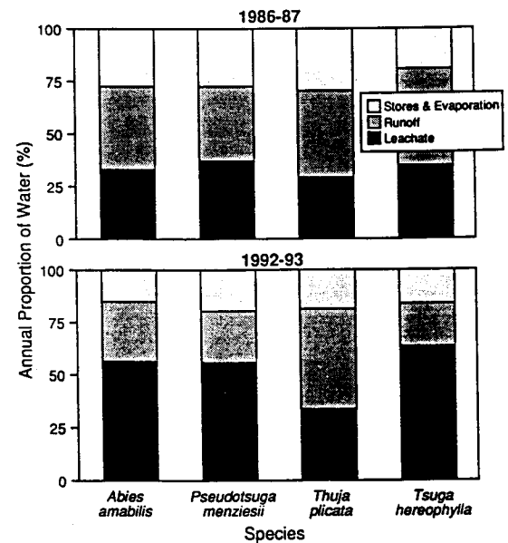
Fig. 3. Annual proportion of leaching, runoff, and storage and evaporation in four species of conifer logs after 1 and 8 years of decomposition. Total canopy throughfall landing on the logs was estimated to be 1,568 and 1,499 liter \text{m}^{-2} log in years 1 and 8, respectively.
