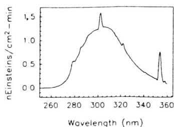
Figure 1. Emission spectrum of Westinghouse FS-40 fluorescent tubes.
