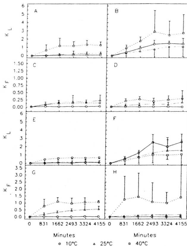
Figure 7. Mean mass balance coefficients, K_L and K_F , at different temperatures and times for triclopyr deposits with Pacific madrone and giant chinkapin leaves. Treatments: (A) K_L madrone, dark; (B) K_L madrone, light; (C) K_F madrone, dark; (D) K_F madrone, light; (E) K_L chinkapin, dark; (F) K_L chinkapin, light; (G) K_F chinkapin, dark; (H) K_F chinkapin, light. Vertical bars are half of the 95% confidence intervals.
